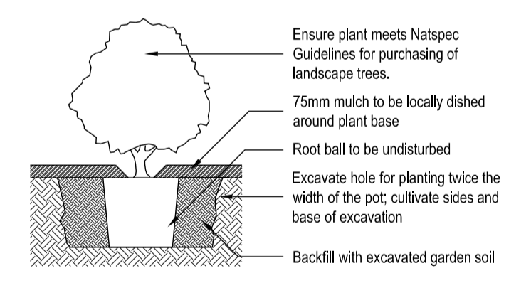
1 Planting Detail NTS Tube, 150mm, 200mm Pot Size
